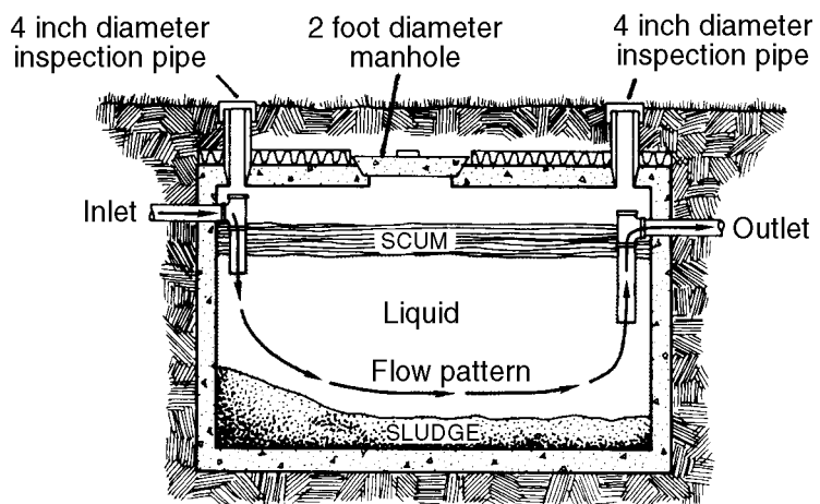
Septic tank cross-section.
