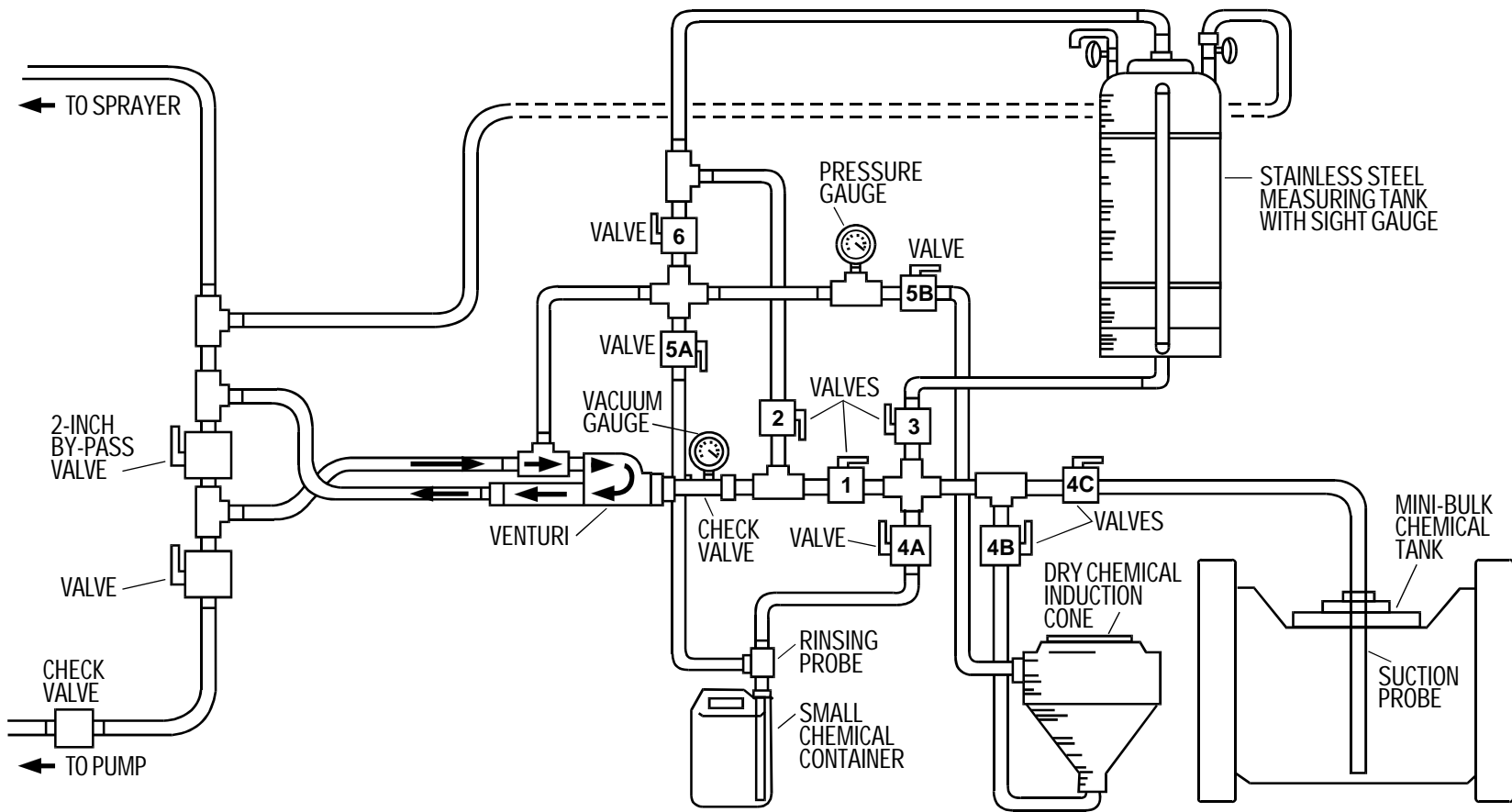
A Vacuum Closed Chemical Handling System
